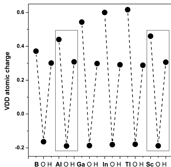
Figure 4. VDD atomic charges of the metal, oxygen, and hydrogen atoms in T_h [\text{M}(\text{H}_2\text{O})_6]^{3+} complexes. The charges for the aluminum and scandium hexaaqua complexes are shown in boxes.
